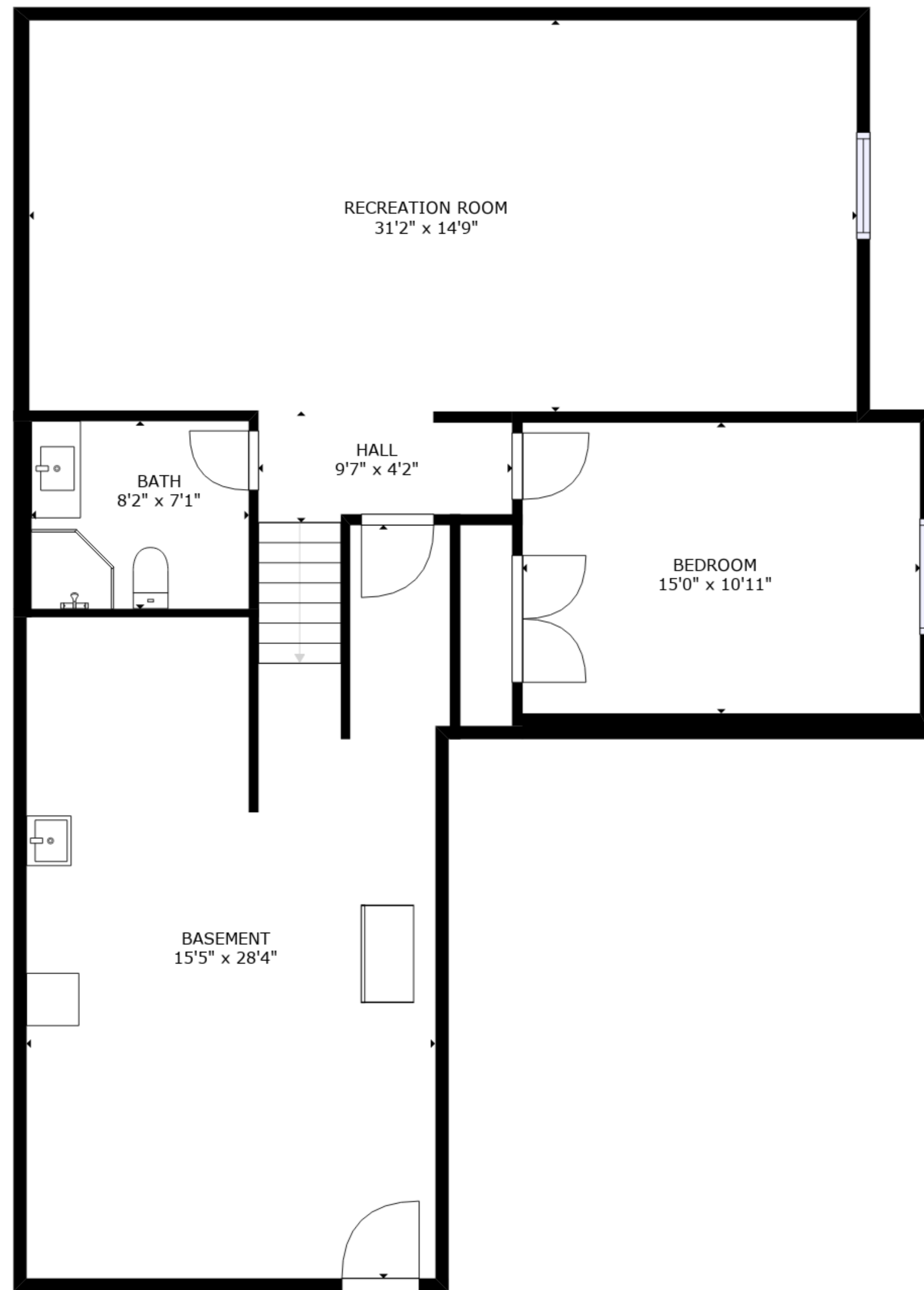
FLOOR 1
