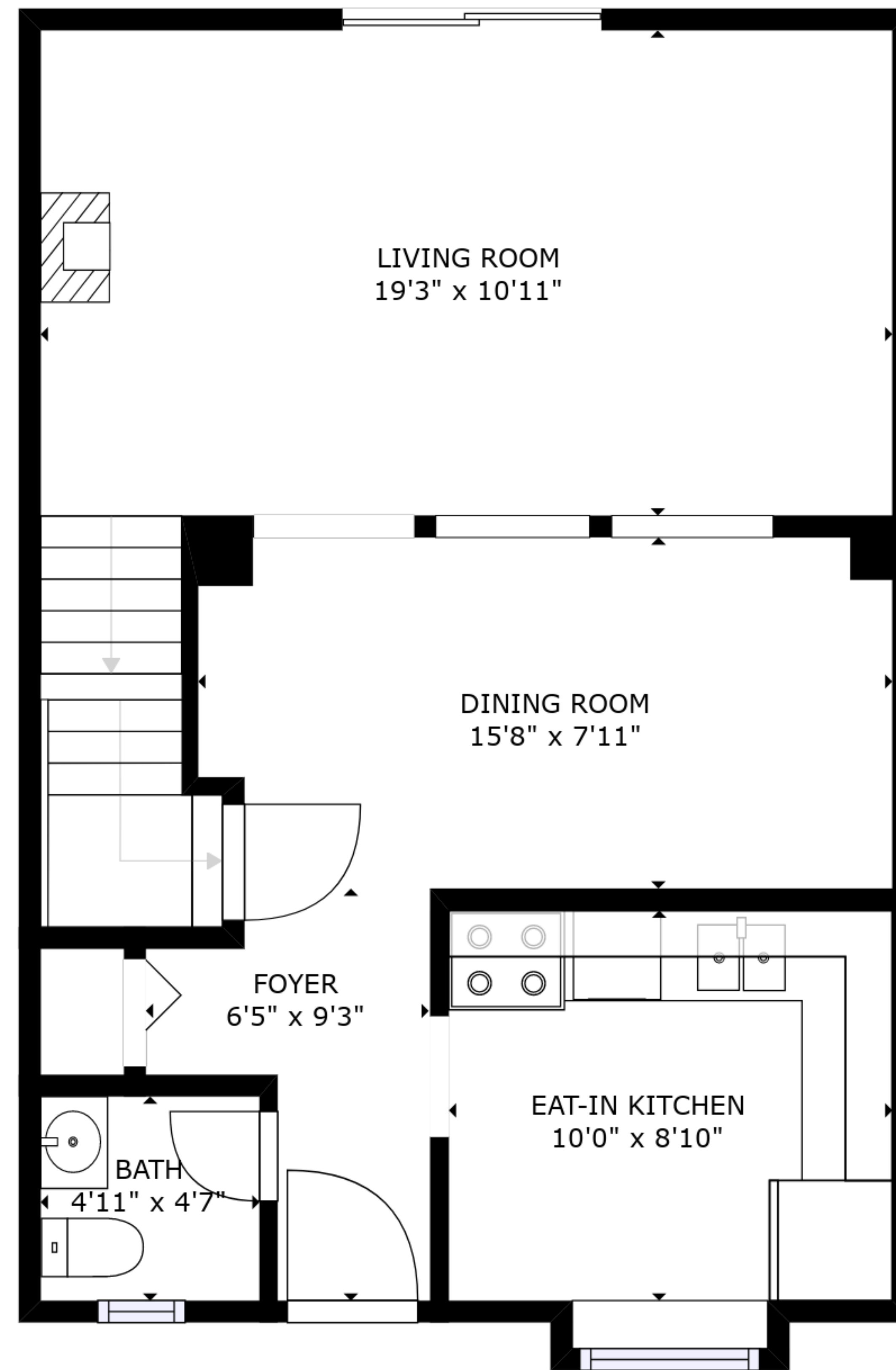
FLOOR 2
