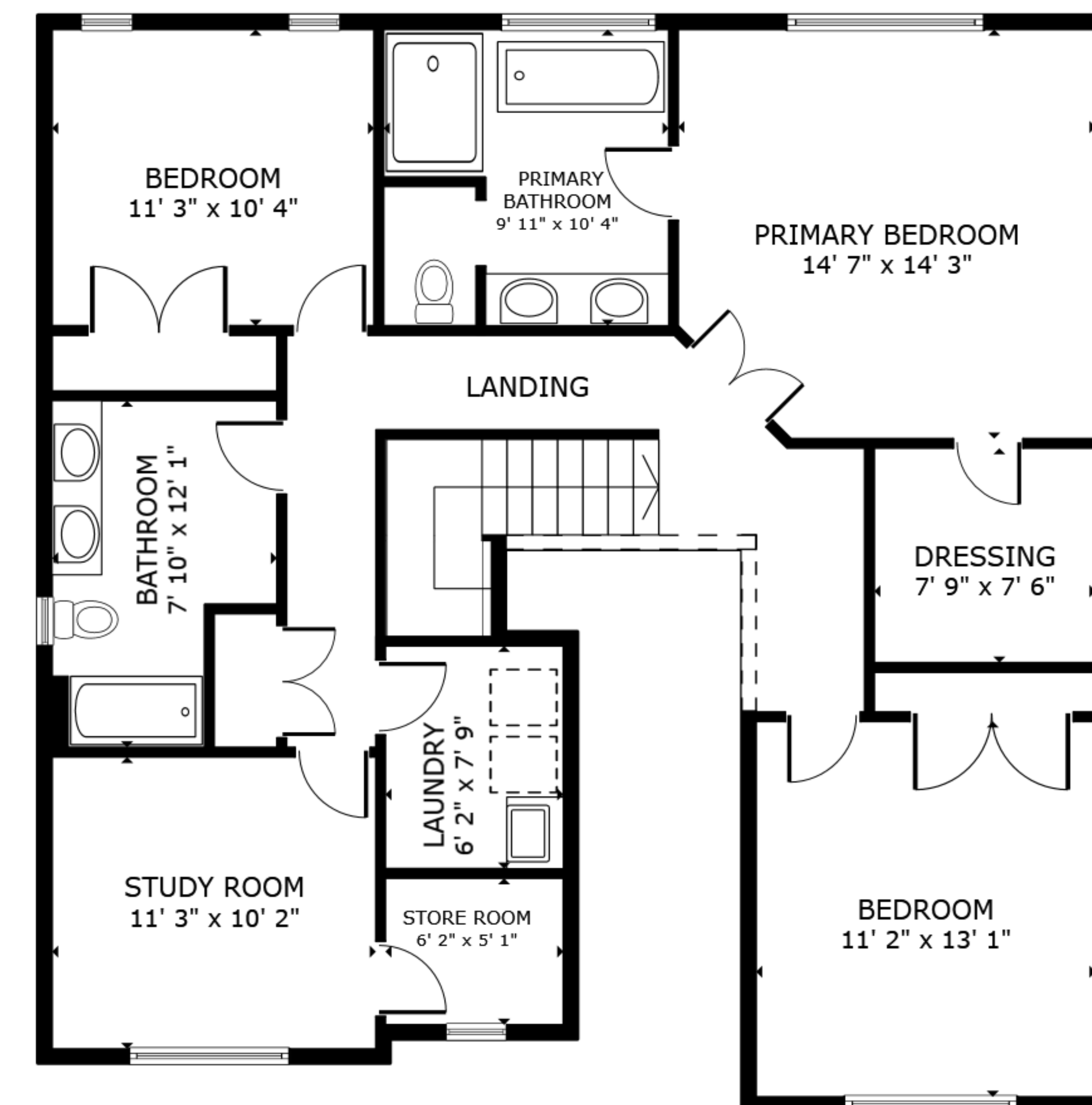
FLOOR 3
